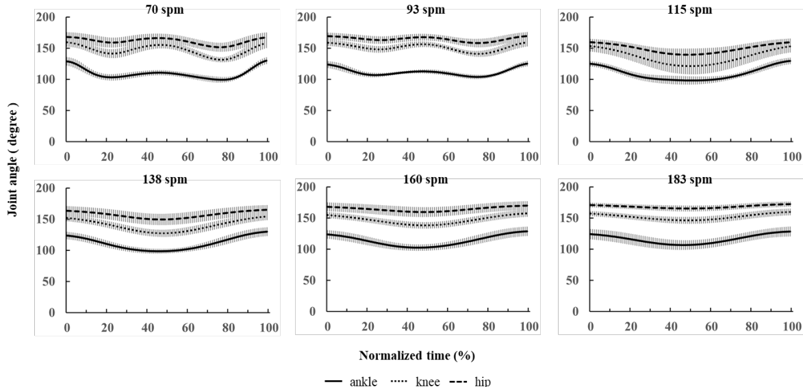
Fig. 2 Averaged patterns of joint angle during ground contact phase in jump cycles between 70 and 183 bpm
